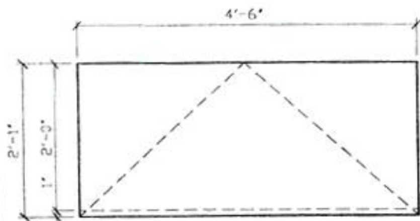
1 TOP VIEW 3/4" = 1'-0"
